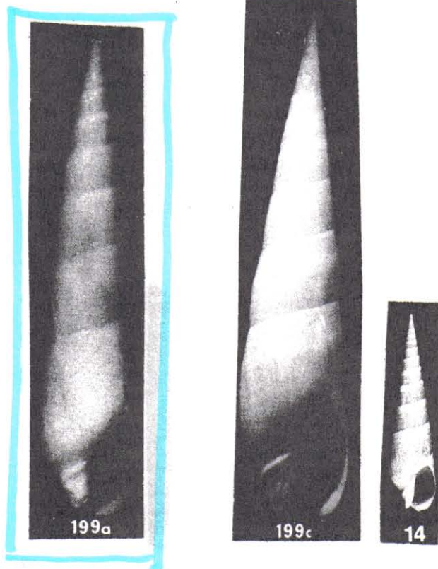
14: Terebra fatua Hinds; Cape Verde Is.; 38.4 mm.
